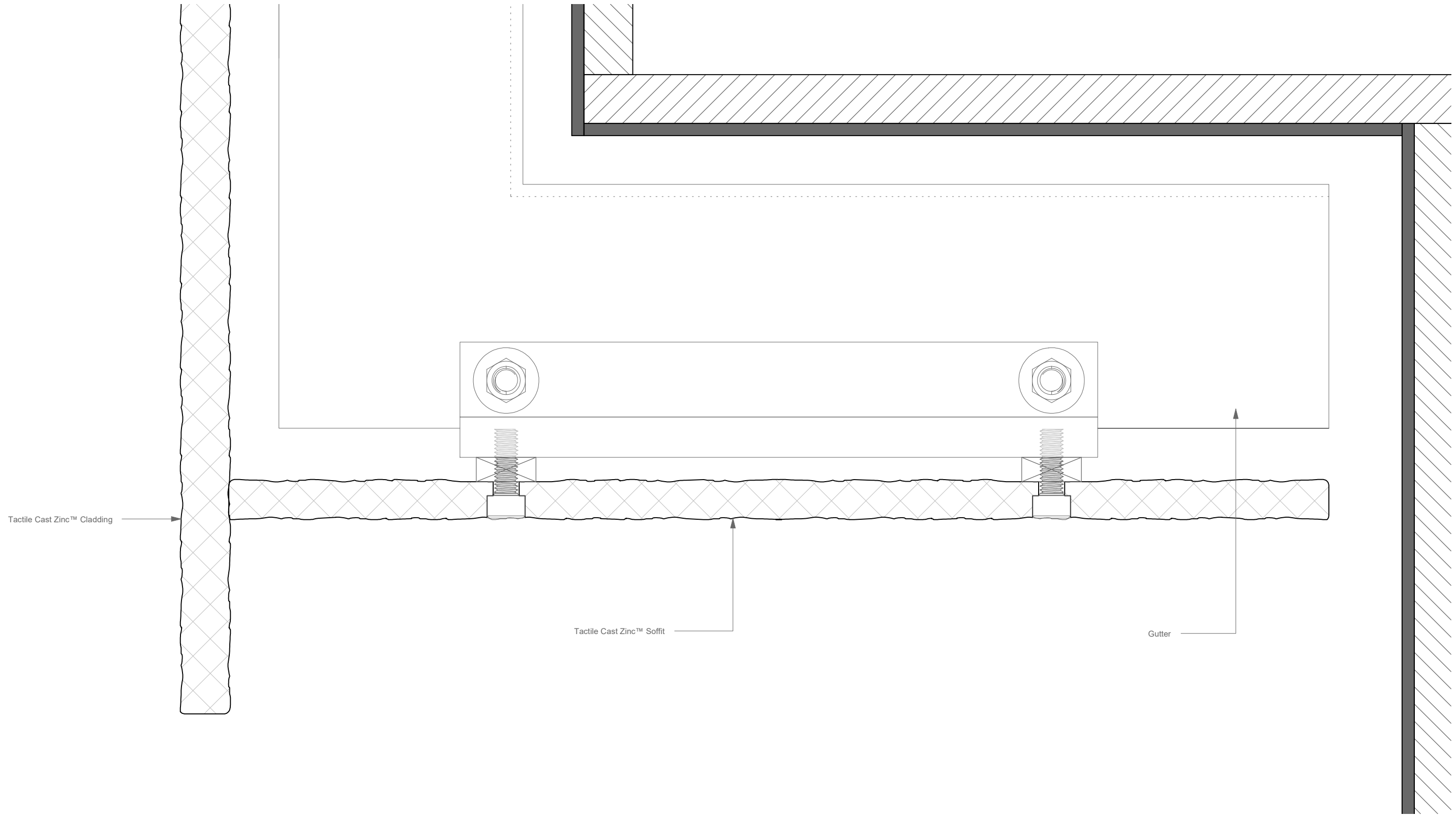
1 Section Detail - Soffit to Vertical Cladding - Tactile Cast Zinc™ Cladding AM-01 Scale: Full Scale
